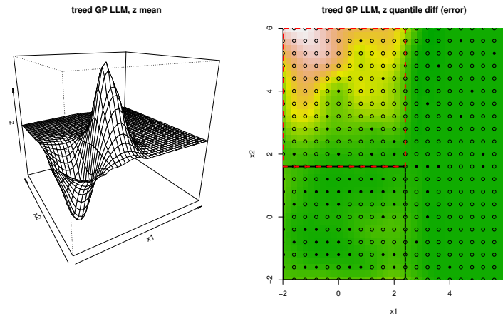
Figure 11: Left : posterior predictive mean using btgp11m on synthetic exponential data; right image plot of posterior predictive variance with data locations X (dots) and predictive locations XX (circles).
