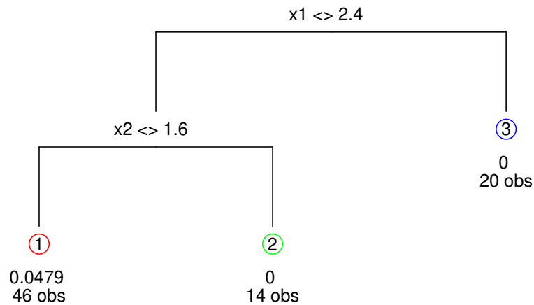
Figure 10: Top-Left : posterior predictive mean using btgp on synthetic exponential data; top-right image plot of posterior predictive variance with data locations \mathbf{X} (dots) and predictive locations \mathbf{XX} (circles). Bottom : MAP trees of each height encountered in the Markov chain with \hat{\sigma}^2 and the number of observations n at the leaves.
