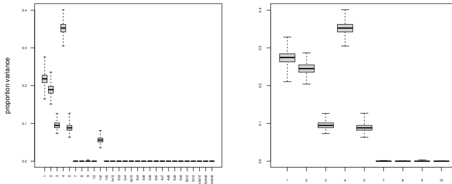
Figure 6: BASS sensitivity analysis – Friedman function.
