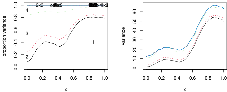
Figure 17: Functional sensitivity analysis, PCA space – Friedman function with functional response.
