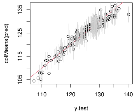
Figure 18: Prediction performance – air foil data.
