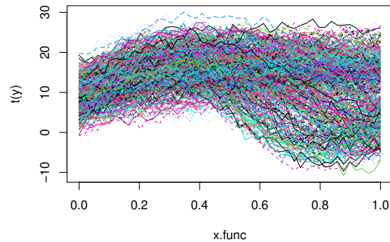
Figure 13: 500 Functional responses. The goal is to fit a functional nonparametric regression model and perform sensitivity analysis.
