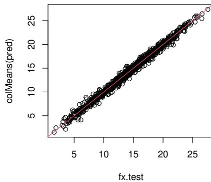
Figure 5: BASS prediction on test data – Friedman function.
