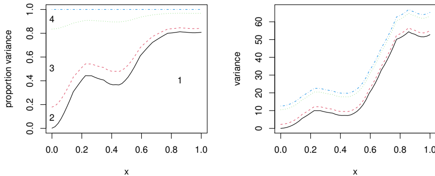
Figure 16: Functional sensitivity analysis – Friedman function with functional response.
