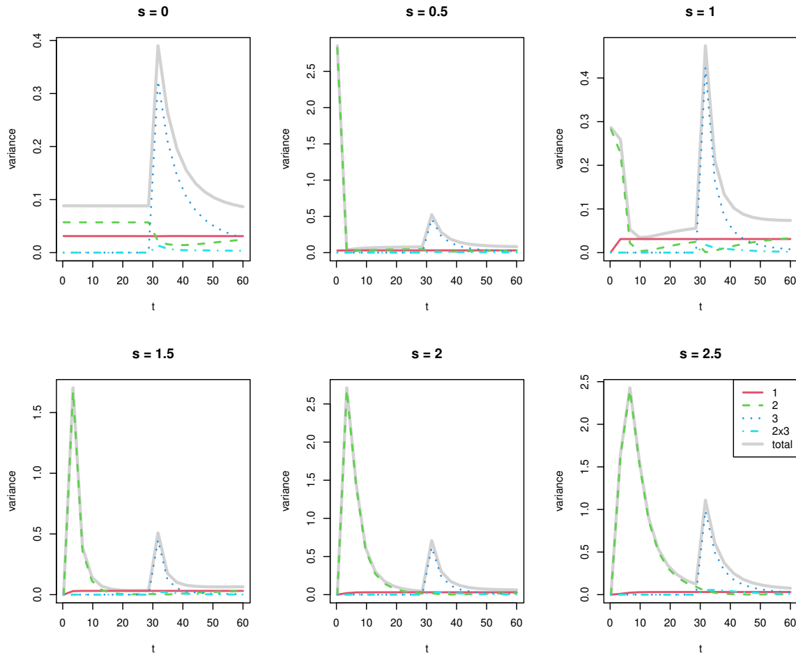
Figure 22: Variance decomposition as a function of space and time – pollutant spill model.
