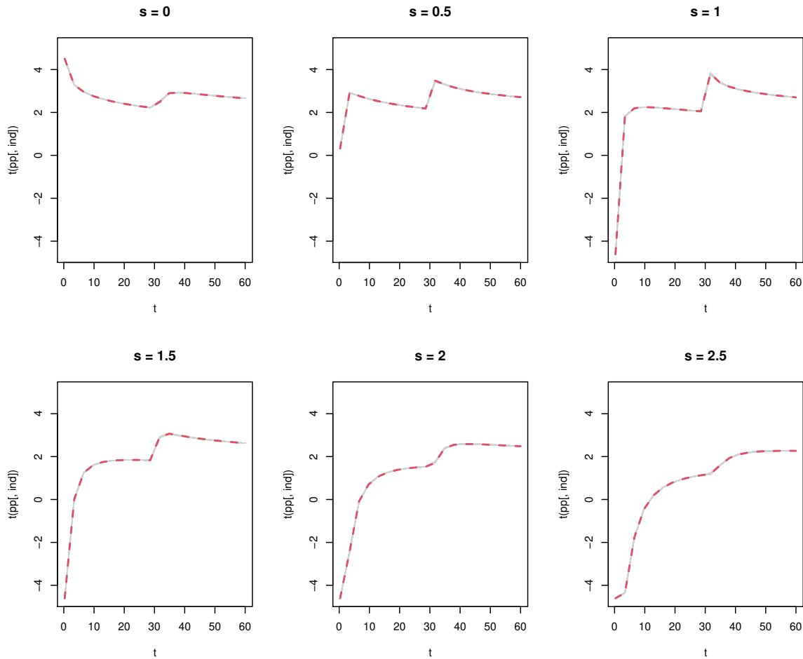
Figure 21: BASS prediction in space and time – pollutant spill model.
