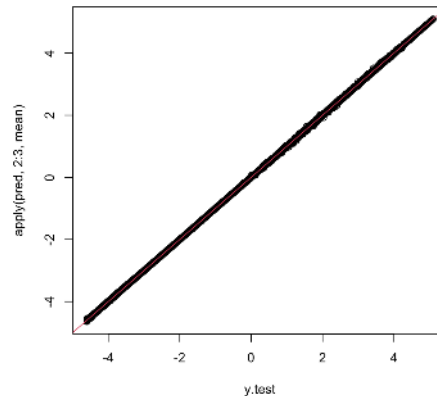
Figure 20: BASS prediction performance – pollutant spill model.
