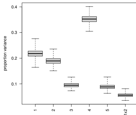
Figure 6: BASS sensitivity analysis – Friedman function.
