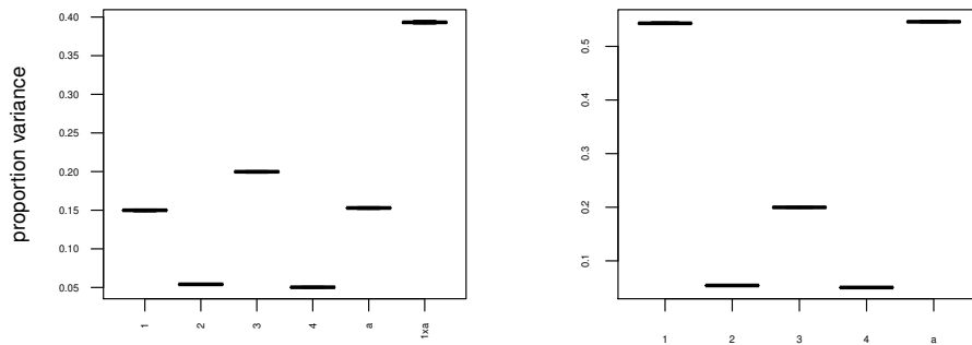
Figure 15: Sensitivity analysis – Friedman function with functional response.
