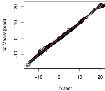
Figure 2: BASS prediction on test data.
