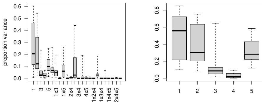
Figure 19: Sobol decomposition – air foil data.
