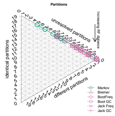
Dataset 98: CI=0.26. Equal weights
