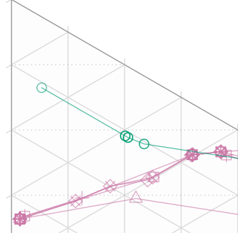
Dataset 75: CI=0.24. Equal weights
