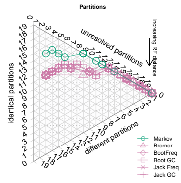
Dataset 34: CI=0.29. Equal weights
