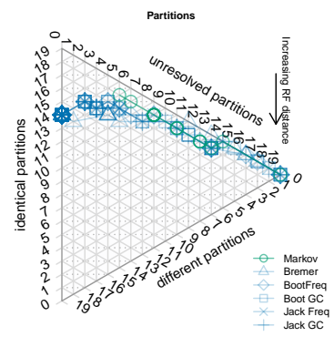
Implied weights (k = 3)
