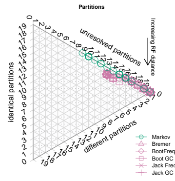
Dataset 8: CI=0.25. Equal weights
