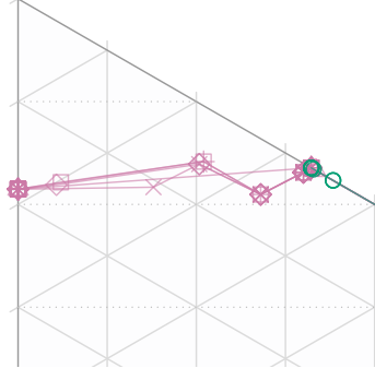
Dataset 51: CI=0.25. Equal weights
