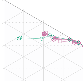
Dataset 57: CI=0.25. Equal weights
