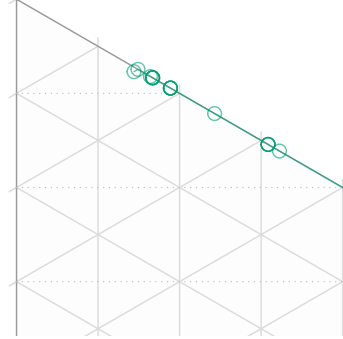
Dataset 13: CI=0.25. Equal weights
