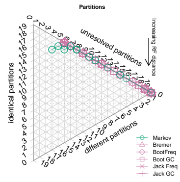
Dataset 56: CI=0.31. Equal weights
