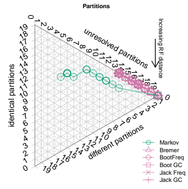
Dataset 97: CI=0.27. Equal weights
