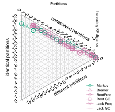
Dataset 21: CI=0.26. Equal weights
