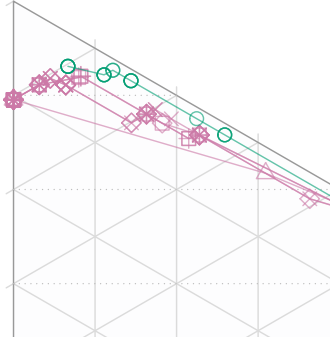
Dataset 32: CI=0.25. Equal weights
