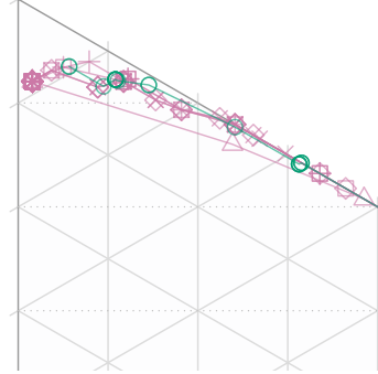
Dataset 69: CI=0.27. Equal weights
