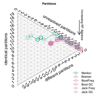
Dataset 36: CI=0.24. Equal weights
