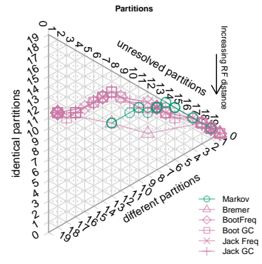
Dataset 5: CI=0.26. Equal weights
