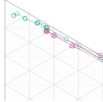
Dataset 95: CI=0.24. Equal weights
