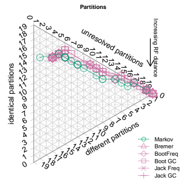
Dataset 96: CI=0.26. Equal weights
