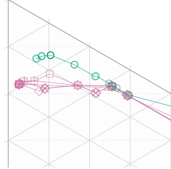
Dataset 87: CI=0.23. Equal weights
