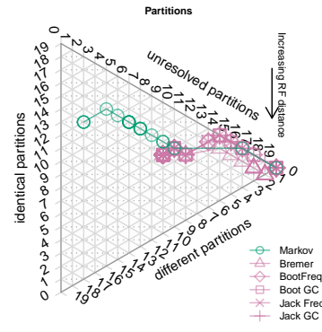
Dataset 53: CI=0.25. Equal weights
