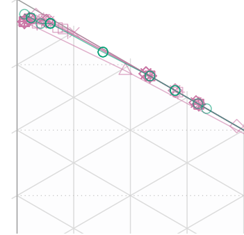
Dataset 18: CI=0.28. Equal weights
