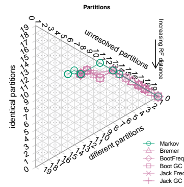
Dataset 28: CI=0.27. Equal weights
