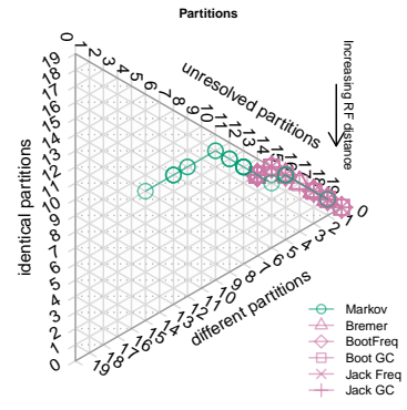
Dataset 15: CI=0.25. Equal weights
