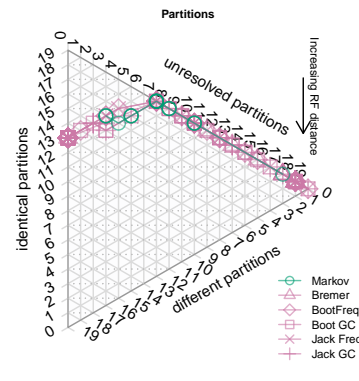
Dataset 55: CI=0.25. Equal weights
