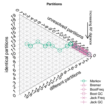
Dataset 30: CI=0.25. Equal weights
