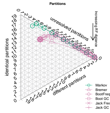
Dataset 7: CI=0.27. Equal weights
