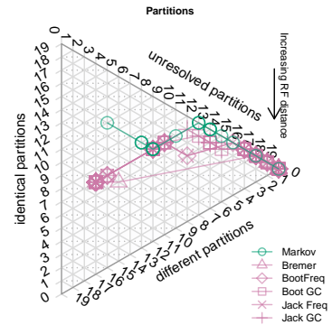
Dataset 75: CI=0.24. Equal weights
