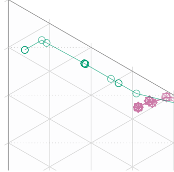
Dataset 53: CI=0.25. Equal weights
