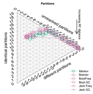
Dataset 86: CI=0.27. Equal weights
