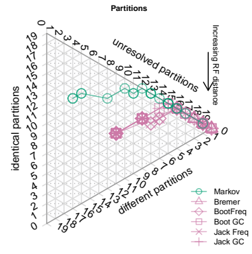
Dataset 99: CI=0.24. Equal weights
