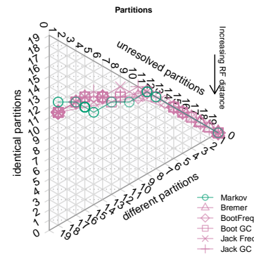
Dataset 26: CI=0.27. Equal weights
