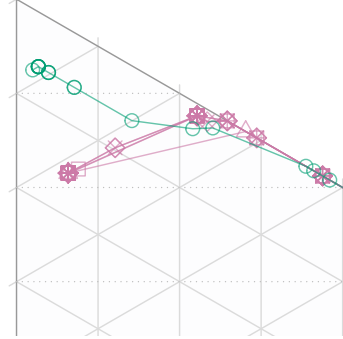
Dataset 37: CI=0.26. Equal weights
