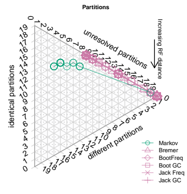
Dataset 64: CI=0.29. Equal weights
