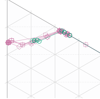
Dataset 93: CI=0.28. Equal weights
