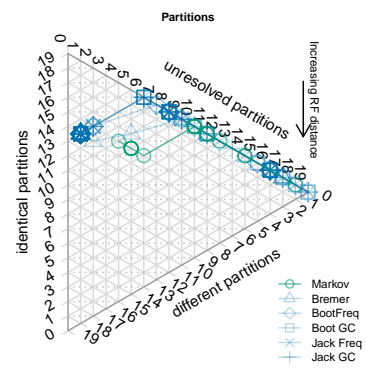
Dataset 50: CI=0.25. Equal weights
