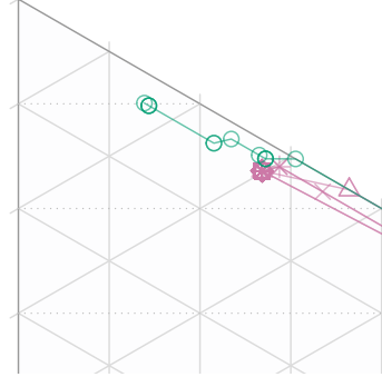
Dataset 55: CI=0.28. Equal weights
