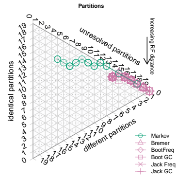
Dataset 33: CI=0.27. Equal weights
