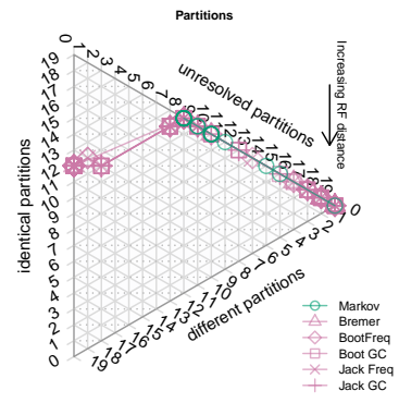
Dataset 51: CI=0.25. Equal weights
