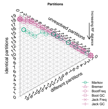
Dataset 6: CI=0.26. Equal weights
