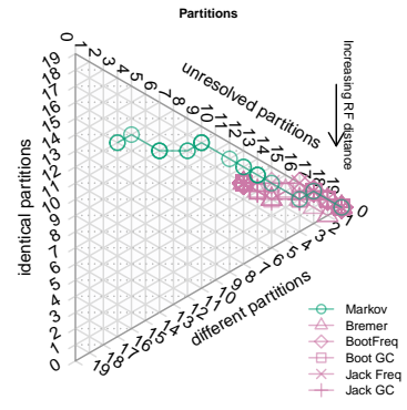
Dataset 95: CI=0.24. Equal weights
