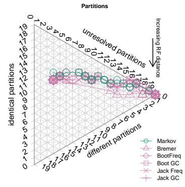
Dataset 59: CI=0.26. Equal weights
