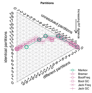
Dataset 63: CI=0.24. Equal weights
