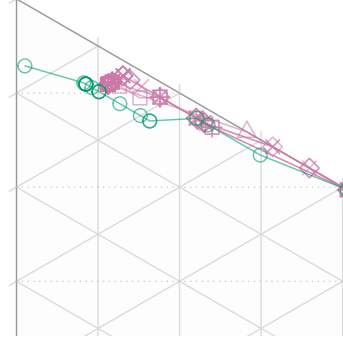
Dataset 96: CI=0.26. Equal weights
