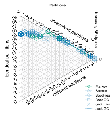
Dataset 56: CI=0.28. Equal weights
