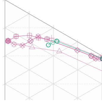
Dataset 5: CI=0.26. Equal weights
