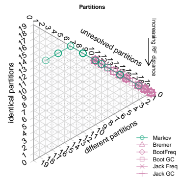
Dataset 66: CI=0.27. Equal weights
