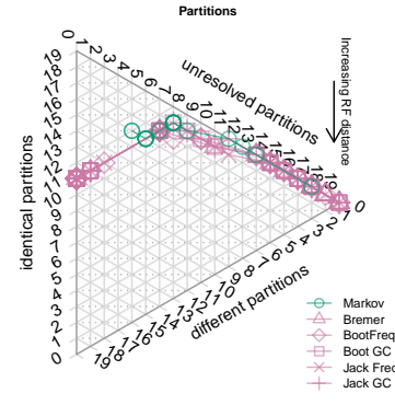
Dataset 25: CI=0.28. Equal weights
