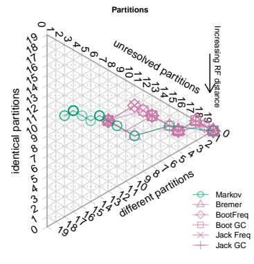
Dataset 76: CI=0.26. Equal weights
