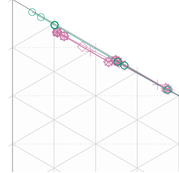
Dataset 46: CI=0.24. Equal weights
