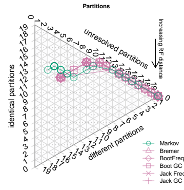
Dataset 37: CI=0.26. Equal weights
