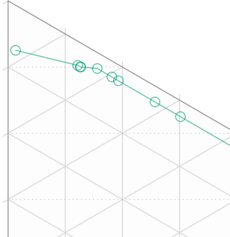
Dataset 92: CI=0.25. Equal weights
