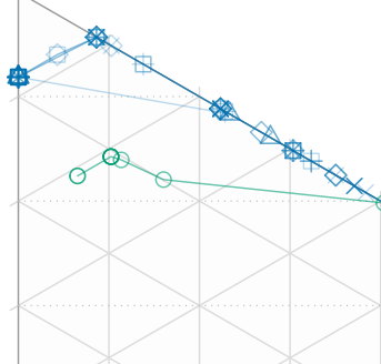
Implied weights (k = 3)
