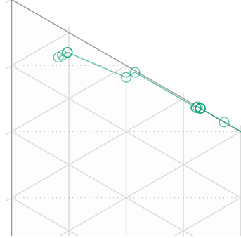
Dataset 99: CI=0.24. Equal weights
