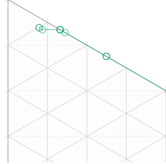
Dataset 23: CI=0.25. Equal weights
