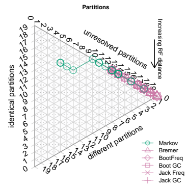
Dataset 44: CI=0.27. Equal weights
