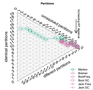
Dataset 92: CI=0.25. Equal weights
