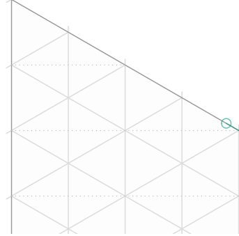
Dataset 67: CI=0.26. Equal weights
