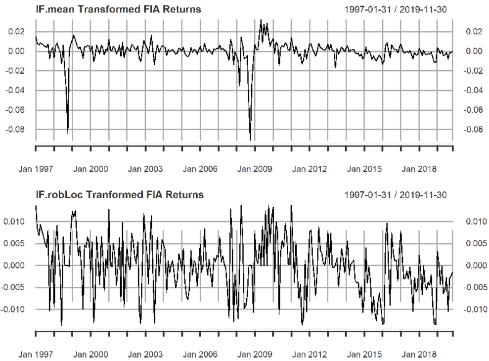
Figure 8: IF.Mean and IF.robMean FIA Transformed FIA Returns
